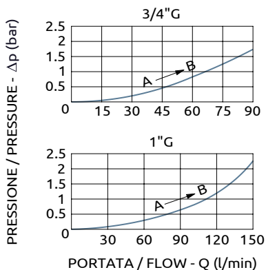
CURVE CARATTERISTICHE PERFORMANCE CURVES
