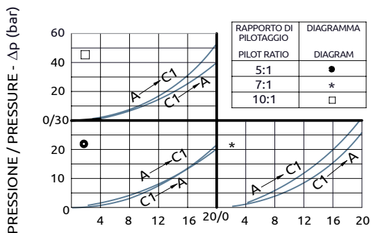
CURVE CARATTERISTICHE PERFORMANCE CURVES
