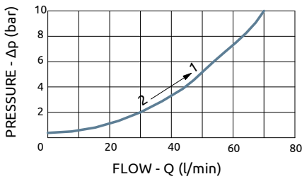
PERFORMANCE CURVES
