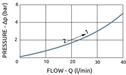
PERFORMANCE CURVES
